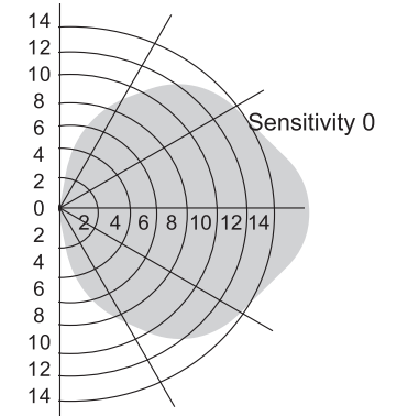
Wall Pattern (Unit: m) Installation Height: 10m
