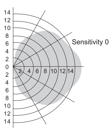
Wall Pattern (Unit: m) Installation Height: 2.5m
