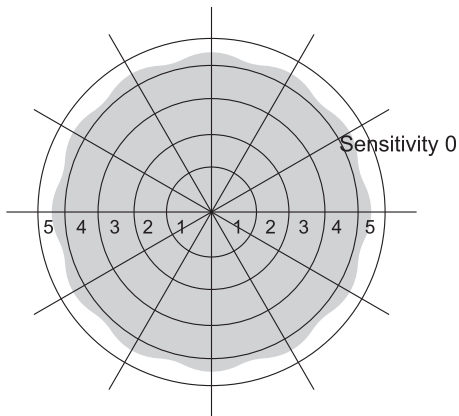
Ceiling Pattern (Unit: m) Installation Height: 2.5m
